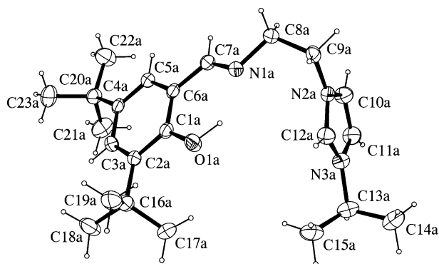
Figure 1. X-ray structure of one crystallographically independent imidazolium cation of [3,5- tert Bu 2 -2-(OH)C 6 H 2 CH=NCH 2 CH 2 -(CH{NCHCHN} i Pr)]Br ( phimid -H·Br). Displacement ellipsoids are drawn at 30% probability level.
