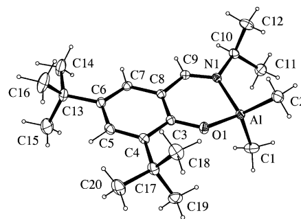
Figure 3. X-ray structure of 1 .
