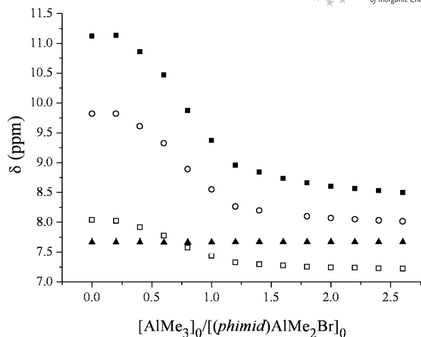
Figure 5. Plot of chemical shifts of \text{H}^1 (■), \text{H}^2 (○), \text{H}^3 (□) and \text{H}^4 (▲) (Scheme 2) for (phimid) - \text{AlMe}_2\text{Br} ( 2 ) versus [\text{AlMe}_3]_0/[(\text{phimid})\text{AlMe}_2\text{Br}]_0 ( \text{C}_6\text{D}_6 , 298 K).
