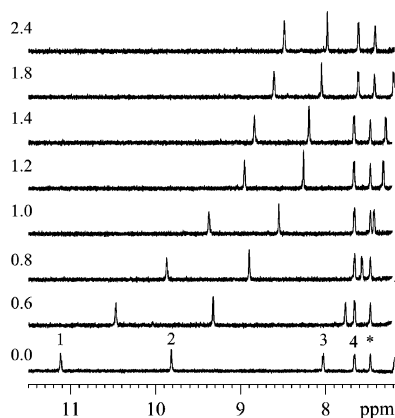
Figure 4. Expanded region of the ^1\text{H} NMR spectra of (phimid) - \text{AlMe}_2\text{Br} at different \text{AlMe}_3/(\text{phimid})\text{AlMe}_2\text{Br} molar ratios. Proton resonances are labeled as in Scheme 2. The asterisk indicates the satellite peak of the deuterated solvent ( \text{C}_6\text{D}_6 , 298 K).
